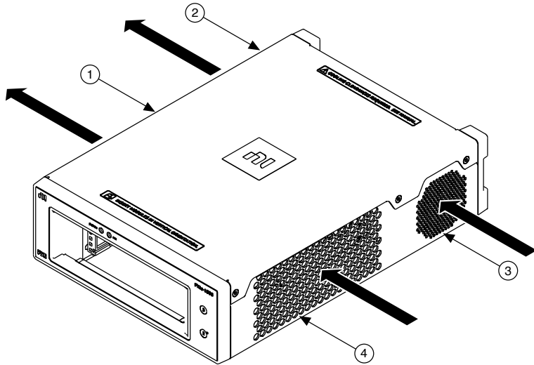
Figure 3. PXIe-1090 Cooling Air Flow
