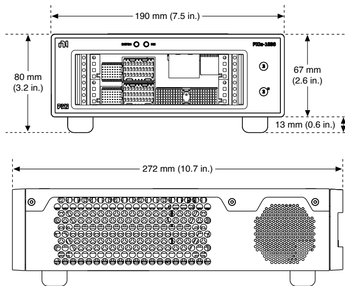
Figure 4. PXIe-1090 Dimensions
