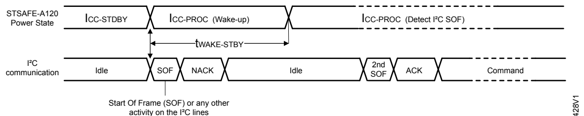
Figure 14. STSAFE-A120 standby entry
