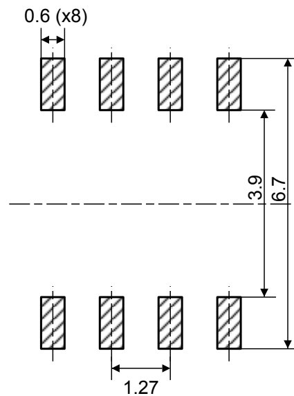
Figure 24. SO8N - footprint example
