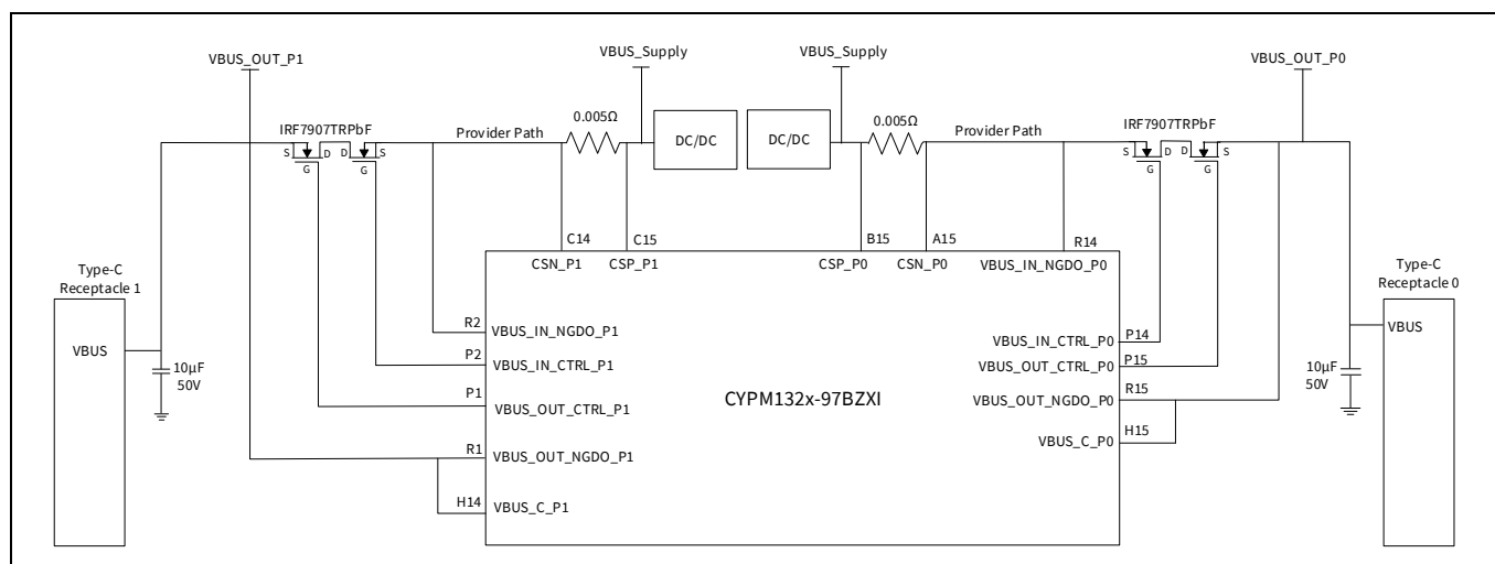
Figure 9 Source configuration on both Type-C ports using 97-ball BGA
