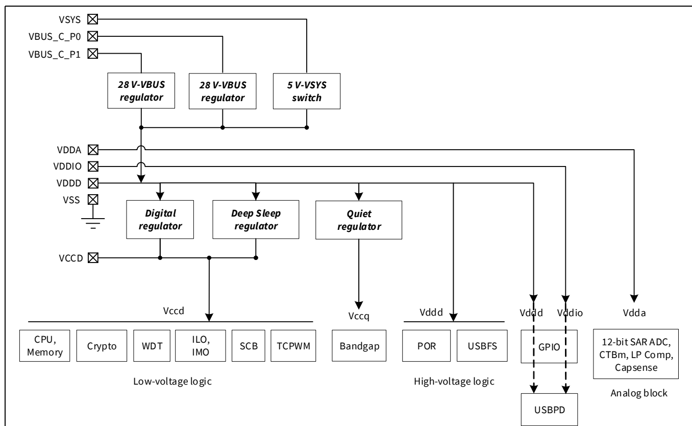
Figure 4 PMG1-S3 power system block diagram
