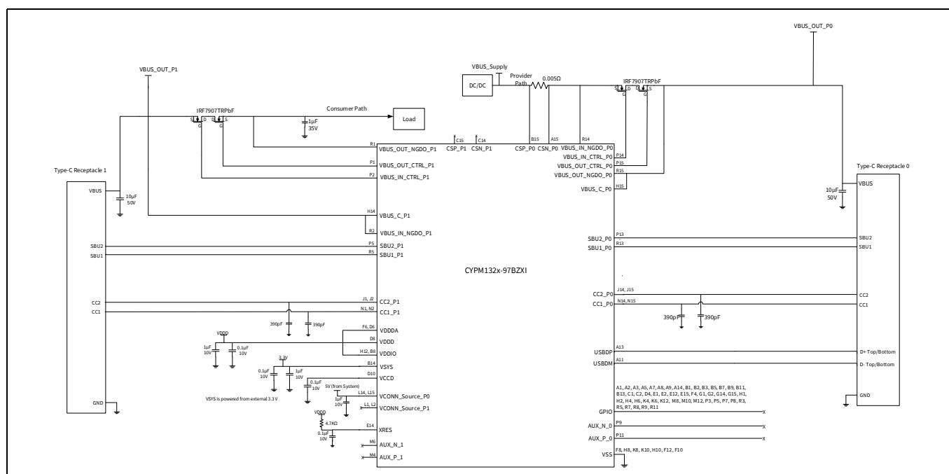
Figure 10 Power provider and consumer application using 97-ball BGA PMG1-S3
