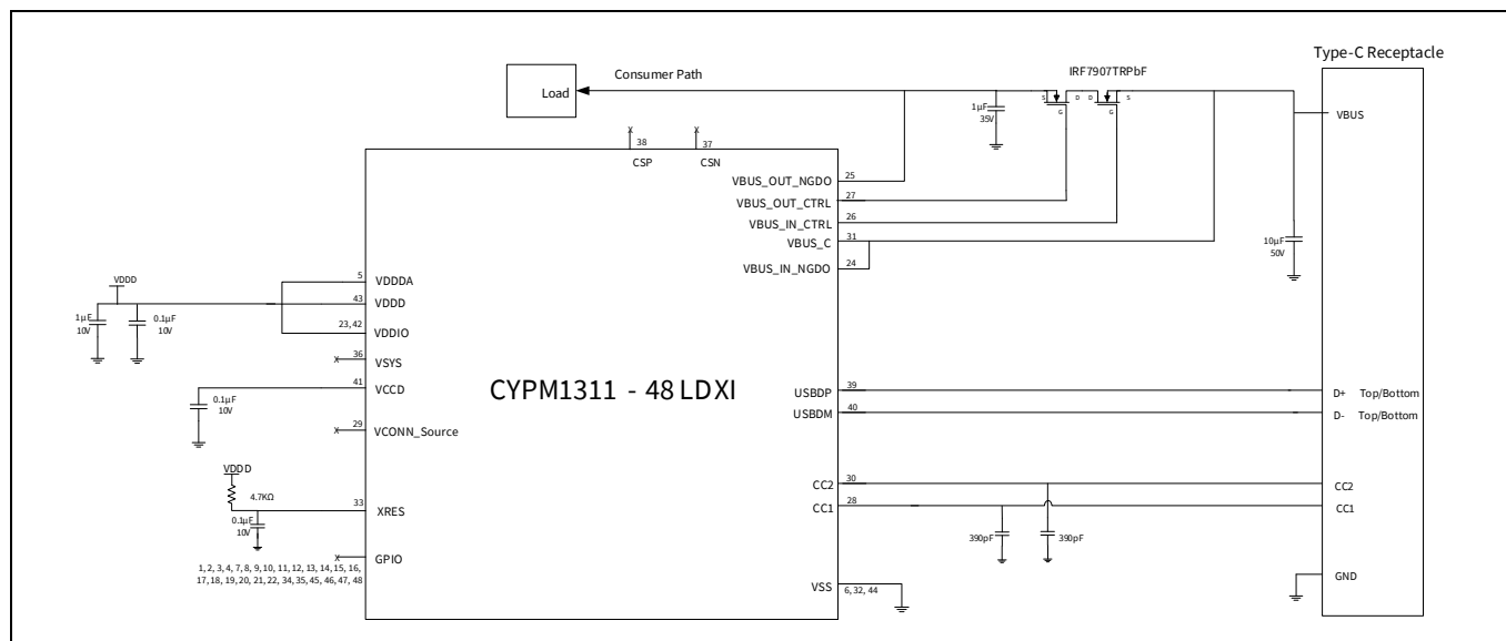
Figure 7 Power sink application using 48-pin QFN PMG1-S3
