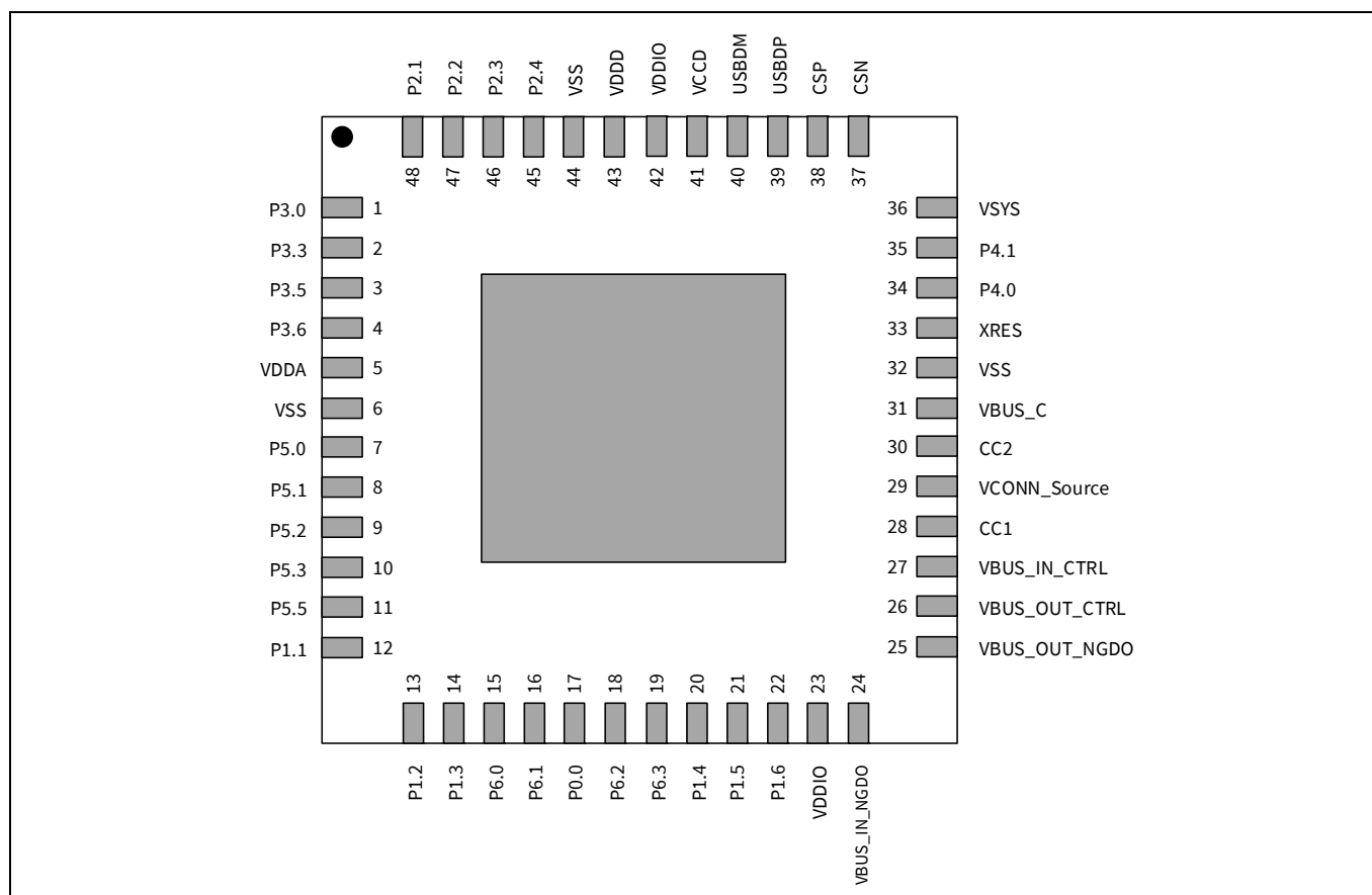
Figure 5 CYPM1311-48LDXI: single-port 48-pin QFN
