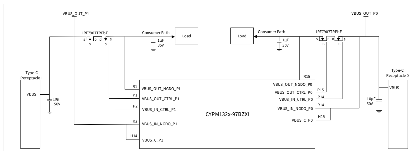
Figure 8 Sink configuration on both Type-C ports using 97-ball BGA
