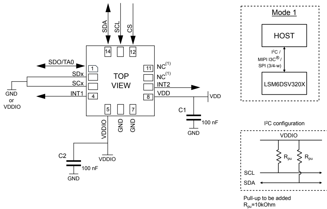
Figure 28. LSM6DSV320X electrical connections in mode 1
