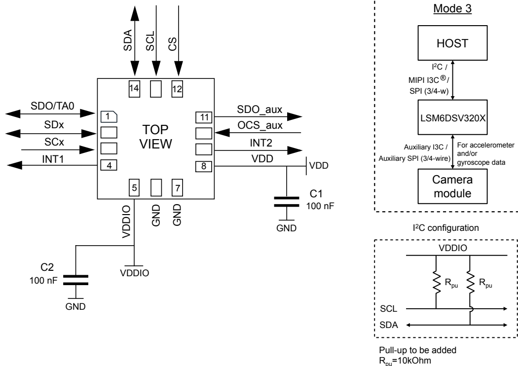
Figure 30. LSM6DSV320X electrical connections in mode 3 (auxiliary 3/4-wire SPI or auxiliary MIPI I3C)
