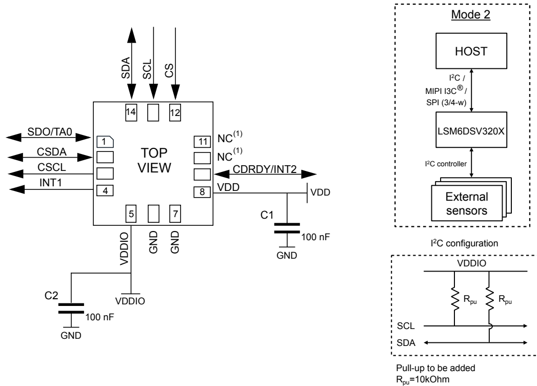
Figure 29. LSM6DSV320X electrical connections in mode 2
