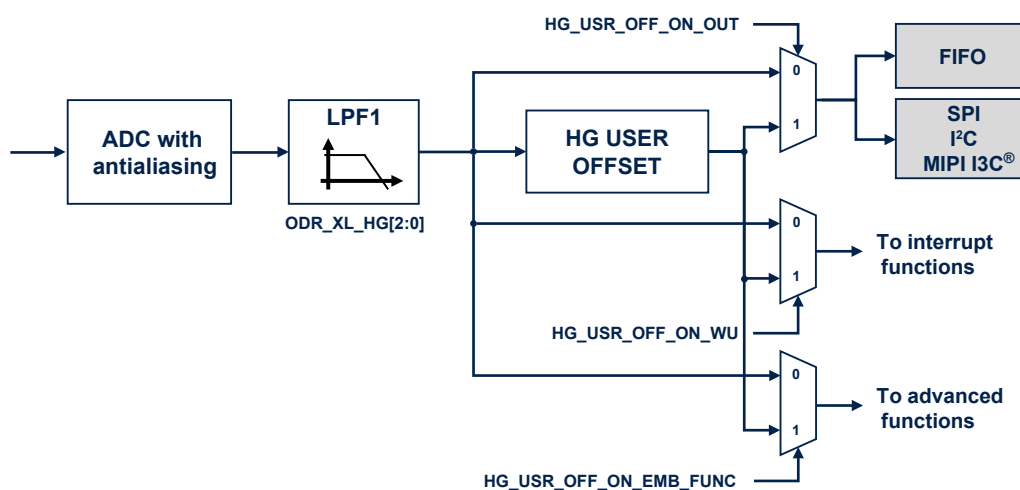
Figure 17. High-g accelerometer filter
