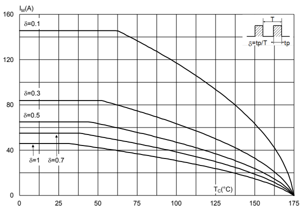
Figure 4. Peak forward current versus case temperature ( f_{\text{sw}} > 10 \text{ kHz} )
