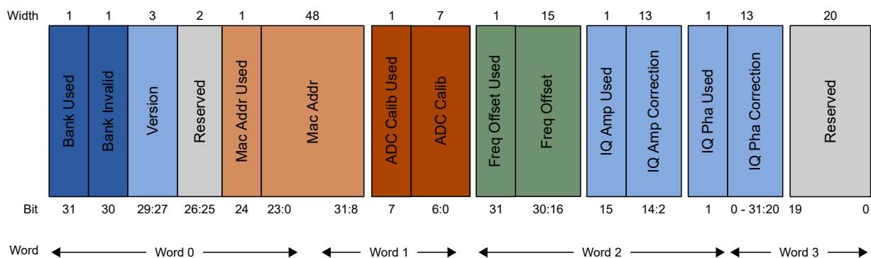
Figure 4-1. Bit map for ATWINC15x0-MR210xB eFuse Bank
