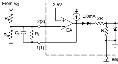
Figure 31-Error Amplifier Compensation
